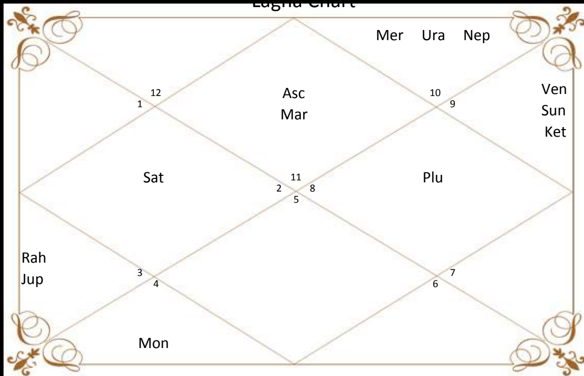
Eighth Chart
