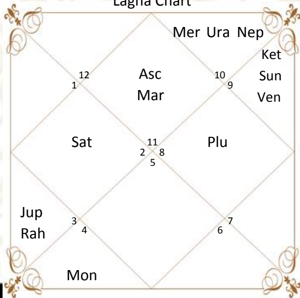
Lagna Chart
