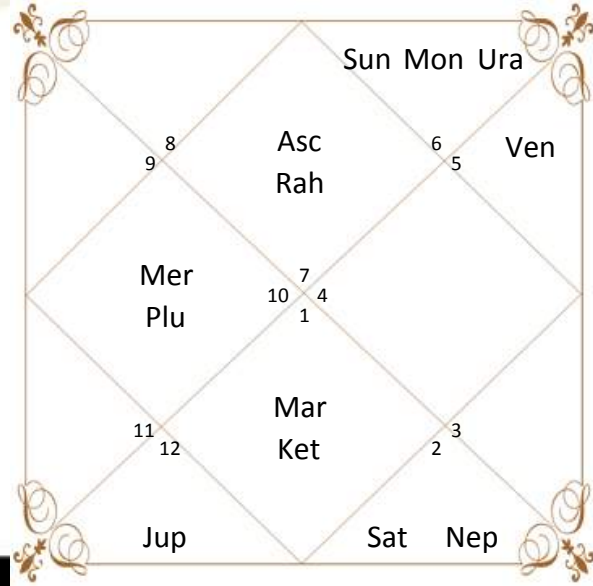
Navamsa
