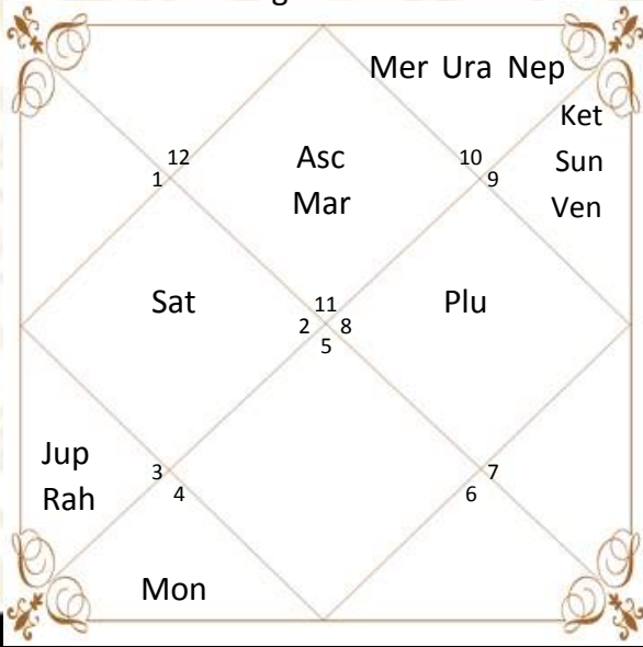
Lagna Chart
