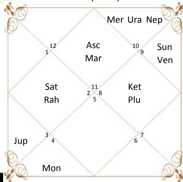
Bhav (Chalit)
