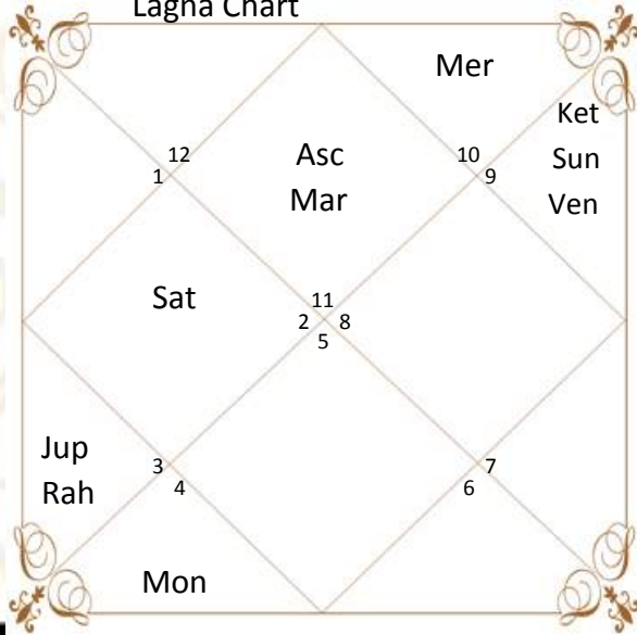
Lagna Chart
